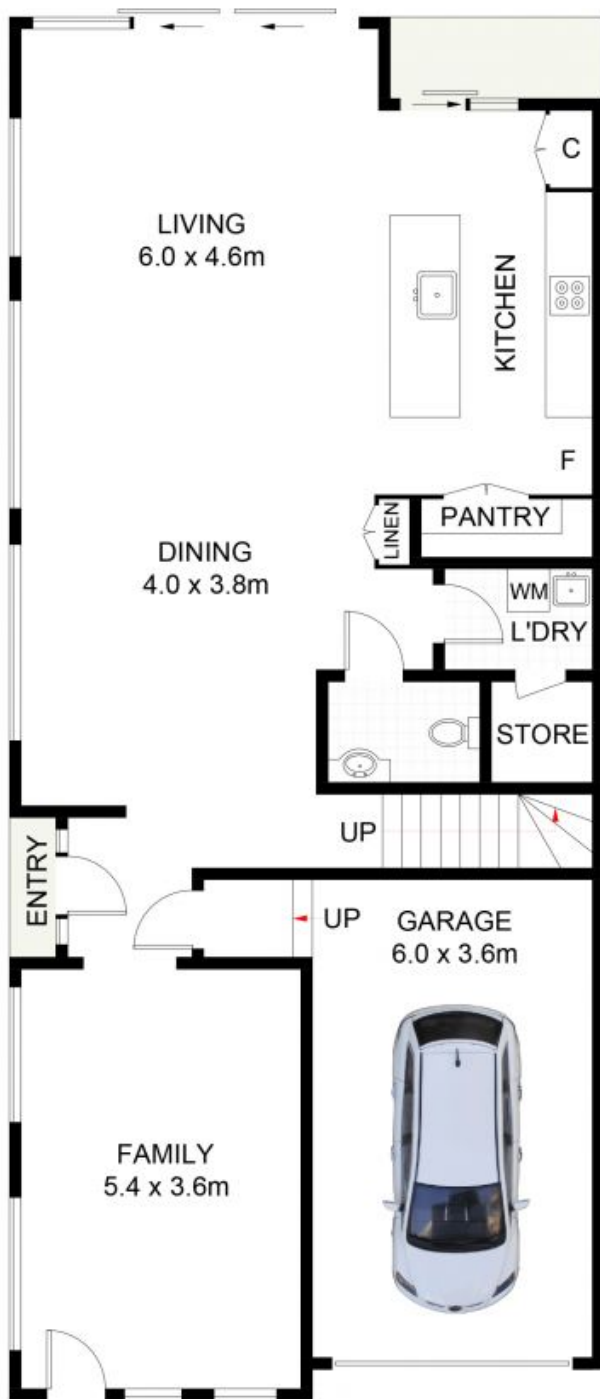
GROUND FLOOR
