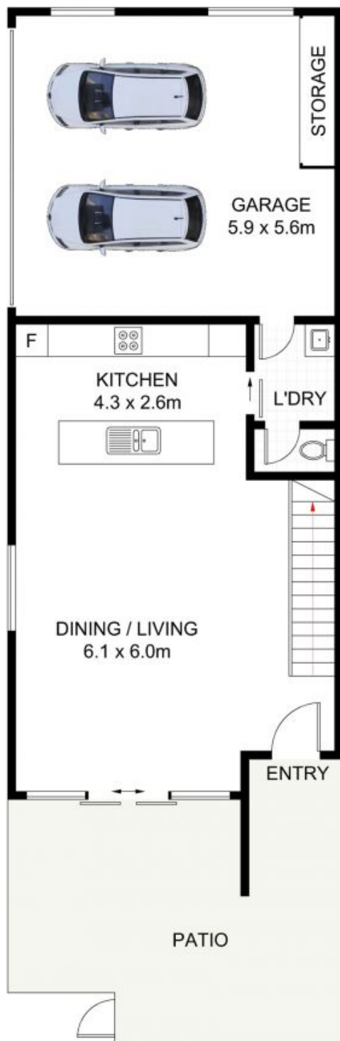
GROUND FLOOR
