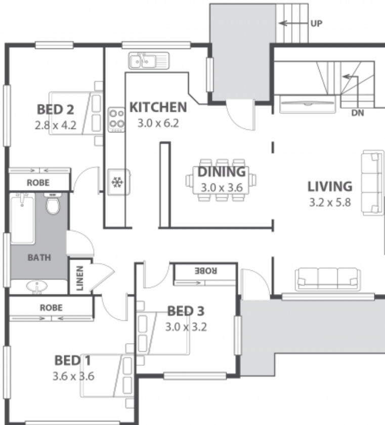
GROUND LEVEL
